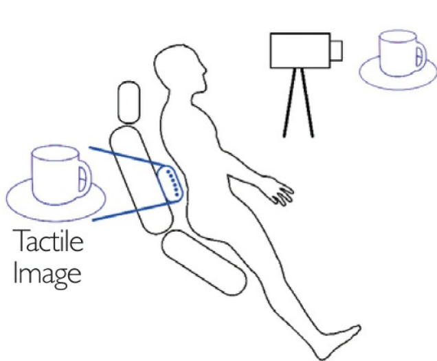
Bach-y-Rita, 1969
